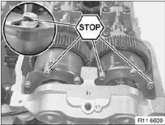
Fig. 296: Identifying Hexagon Socket Screws
