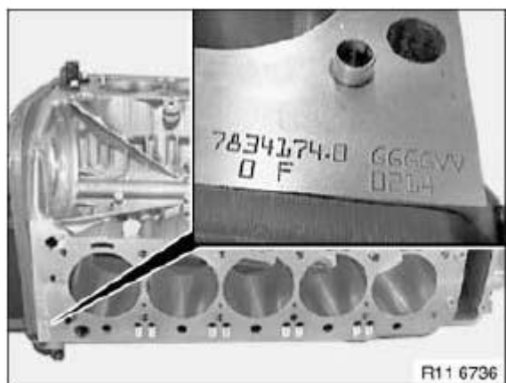
Fig. 125: Identifying Color Allocation On Crankshaft (Crankcase Bearing Block) Courtesy of BMW OF NORTH AMERICA, INC.
