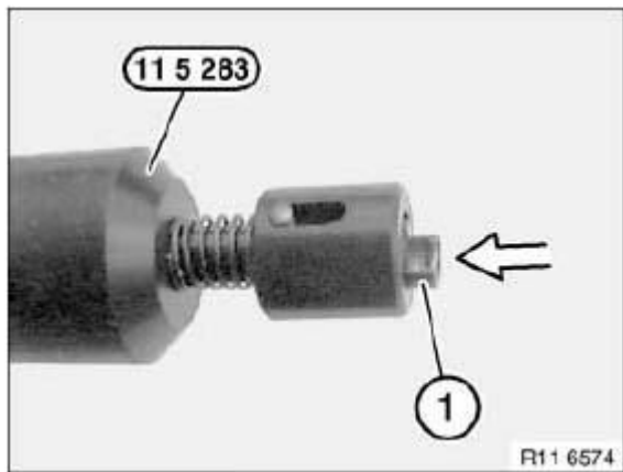
Fig. 263: Pressing Valve Key Into Special Tool 11 5 283 Courtesy of BMW OF NORTH AMERICA, INC.
