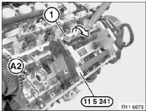
Fig. 202: Relieving Tension On Eccentric Shaft At Hexagon Head
