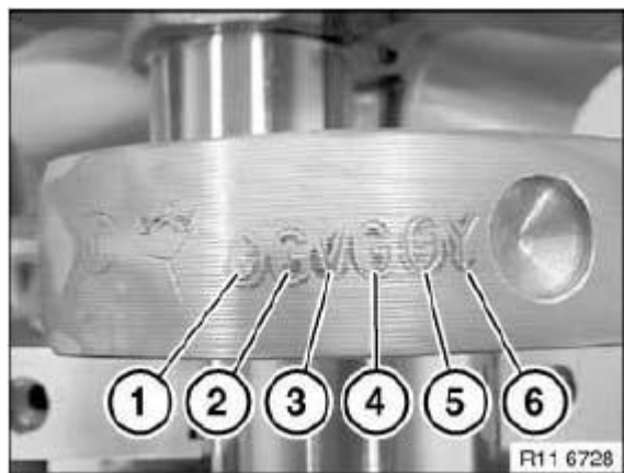
Fig. 124: Identifying Color Allocation On Crankshaft (Bedplate Bearing Block) Courtesy of BMW OF NORTH AMERICA, INC.
