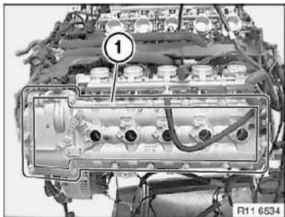
Fig. 42: Identifying Cylinder Head Cover Courtesy of BMW OF NORTH AMERICA, INC.
