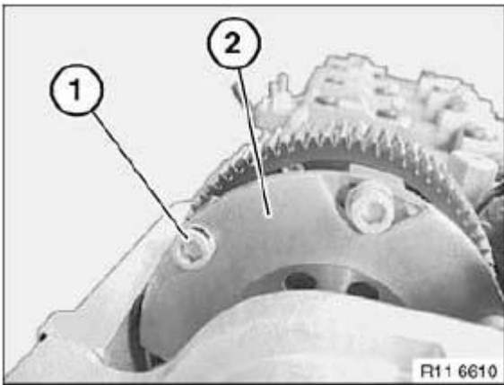
Fig. 297: Identifying Hexagon Socket Screws
