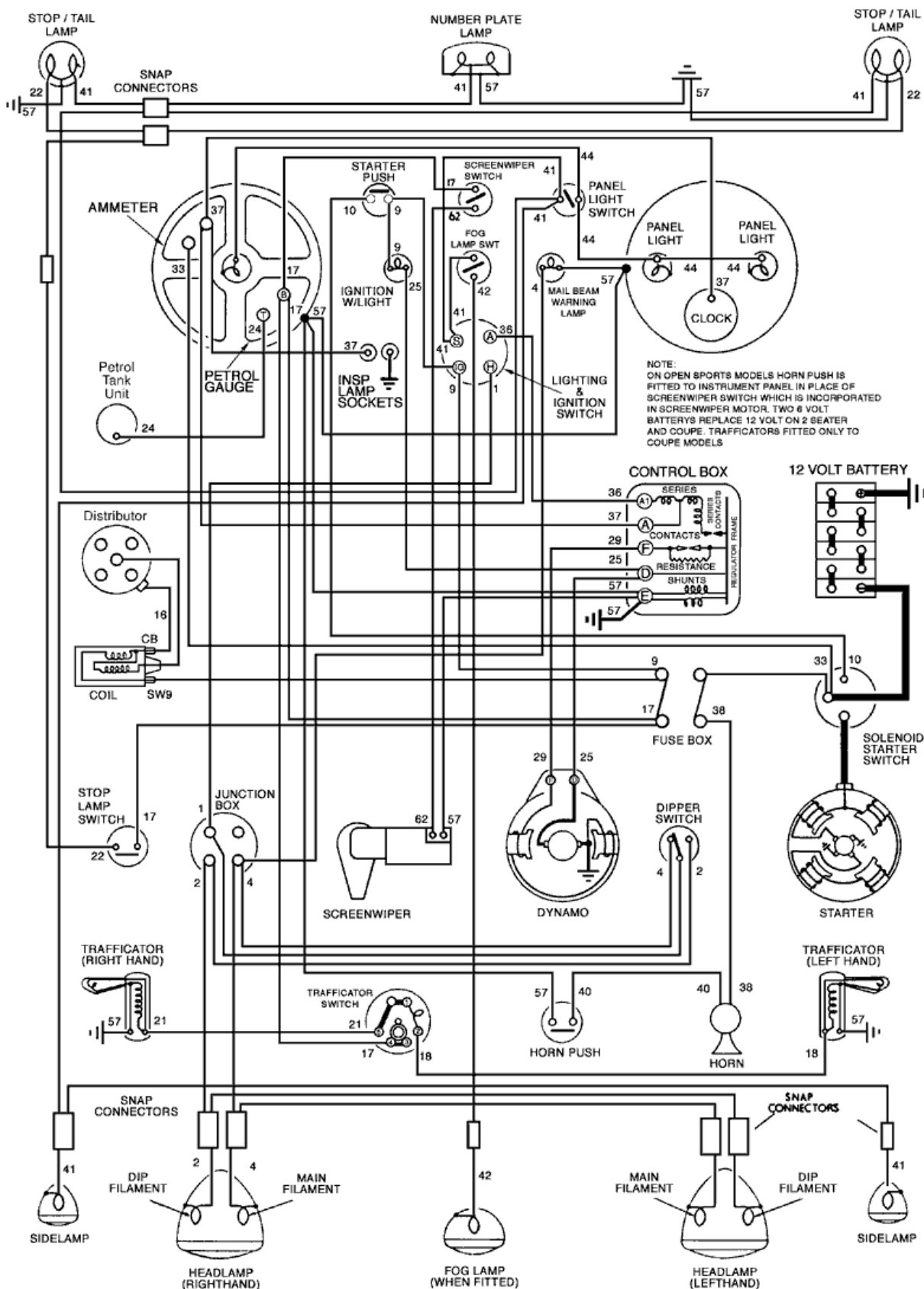
Wiring Diagram Morgan +4 Model 1950-53
