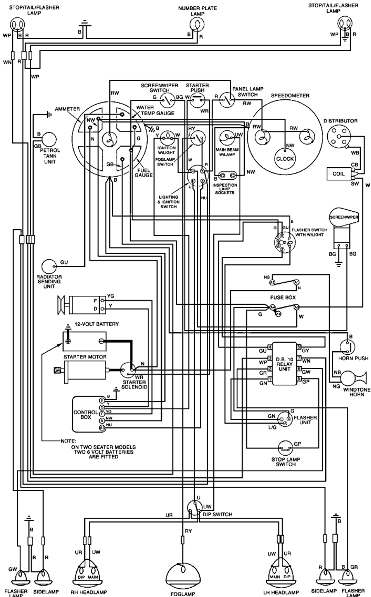
WIRING DIAGRAM MORGAN (1955-58)
