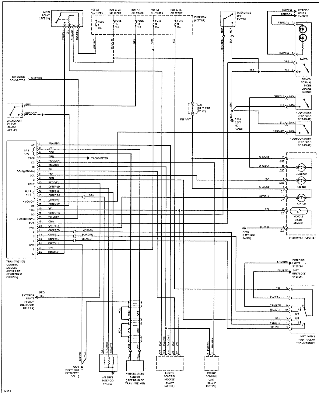
1.6L, 4 Speed A/T Circuit
