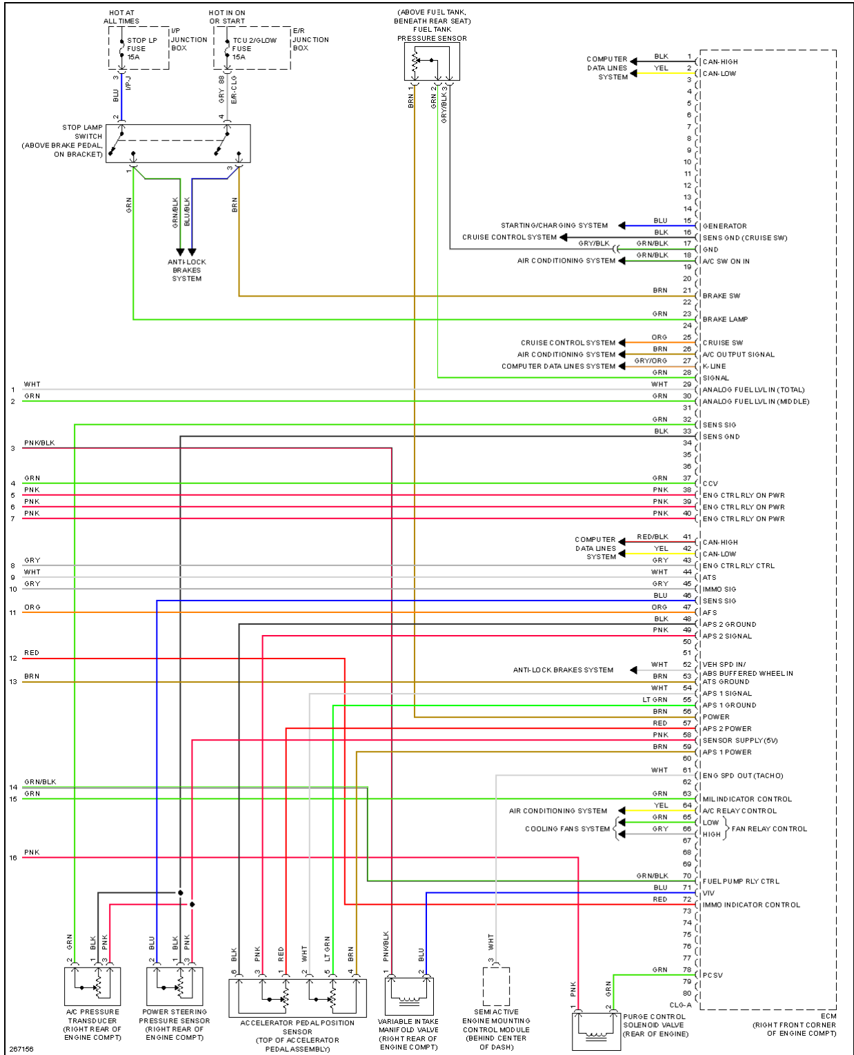
Fig. 22: 3.8L, Engine Performance Circuit (5 of 5)
