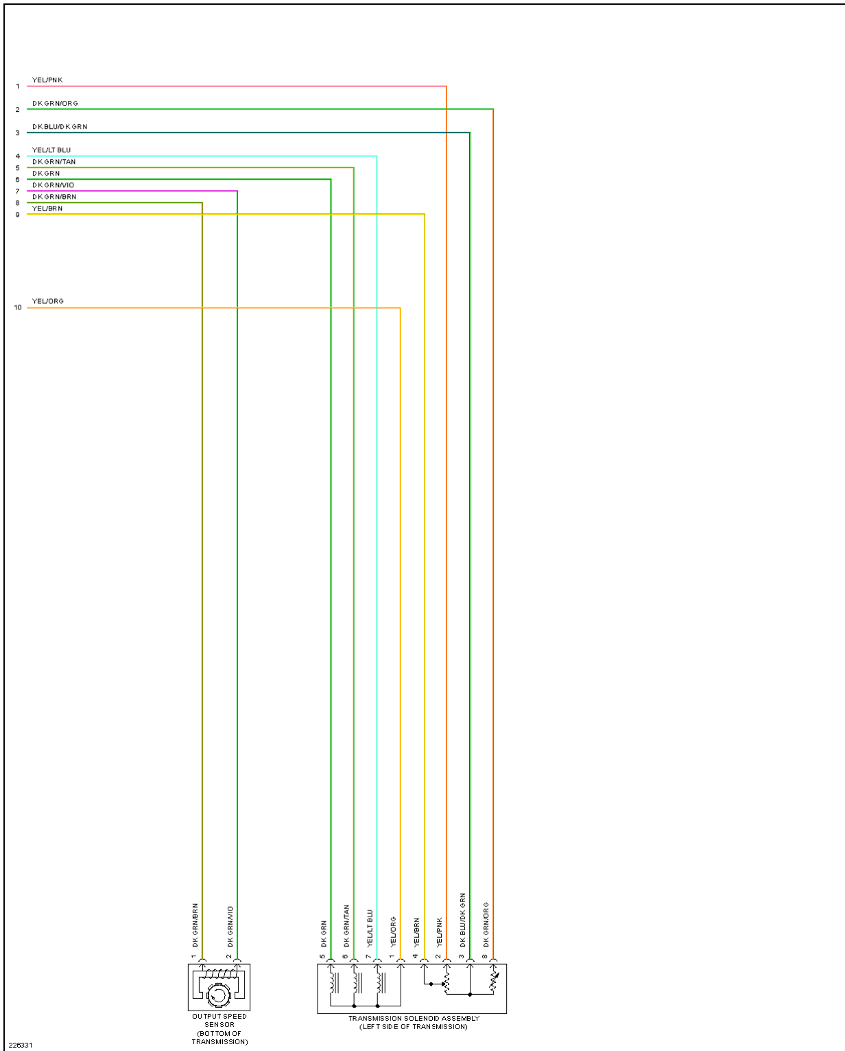
Fig. 20: 5.9L Diesel, Engine Performance Circuit (4 of 4)
