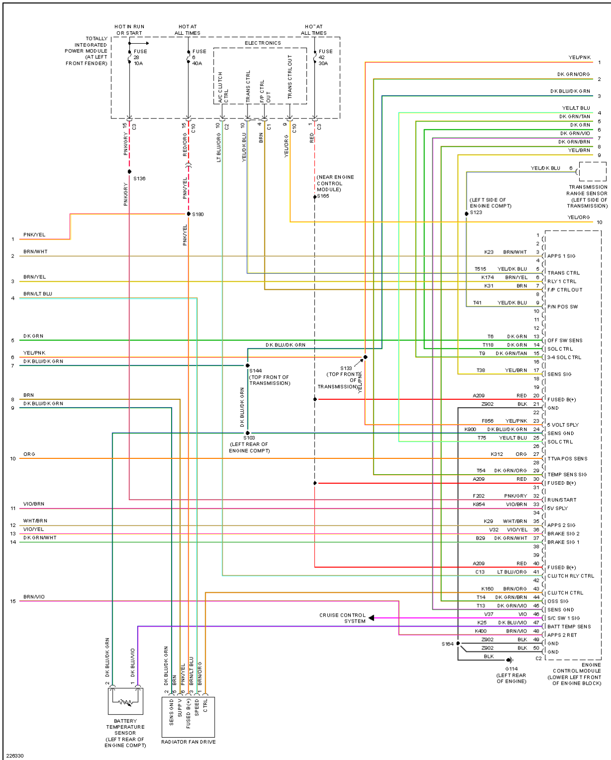
Fig. 19: 5.9L Diesel, Engine Performance Circuit (3 of 4)
