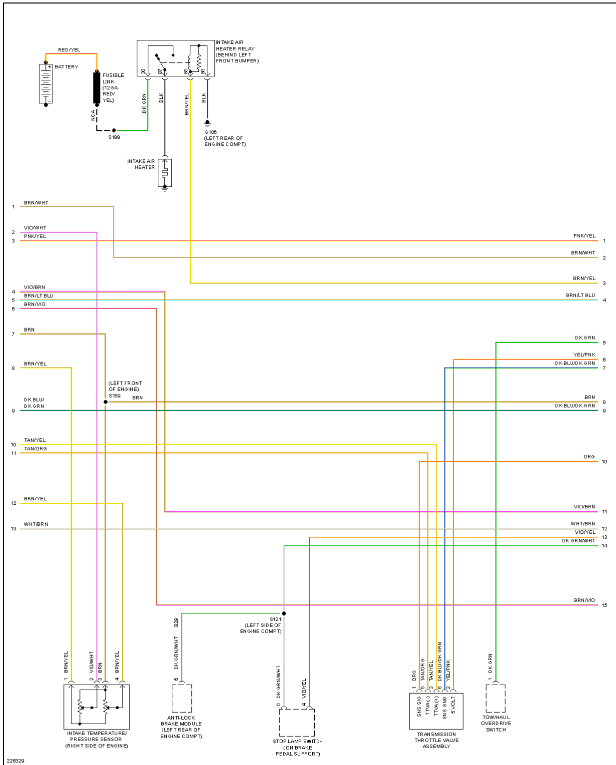
Fig. 18: 5.9L Diesel, Engine Performance Circuit (2 of 4)
