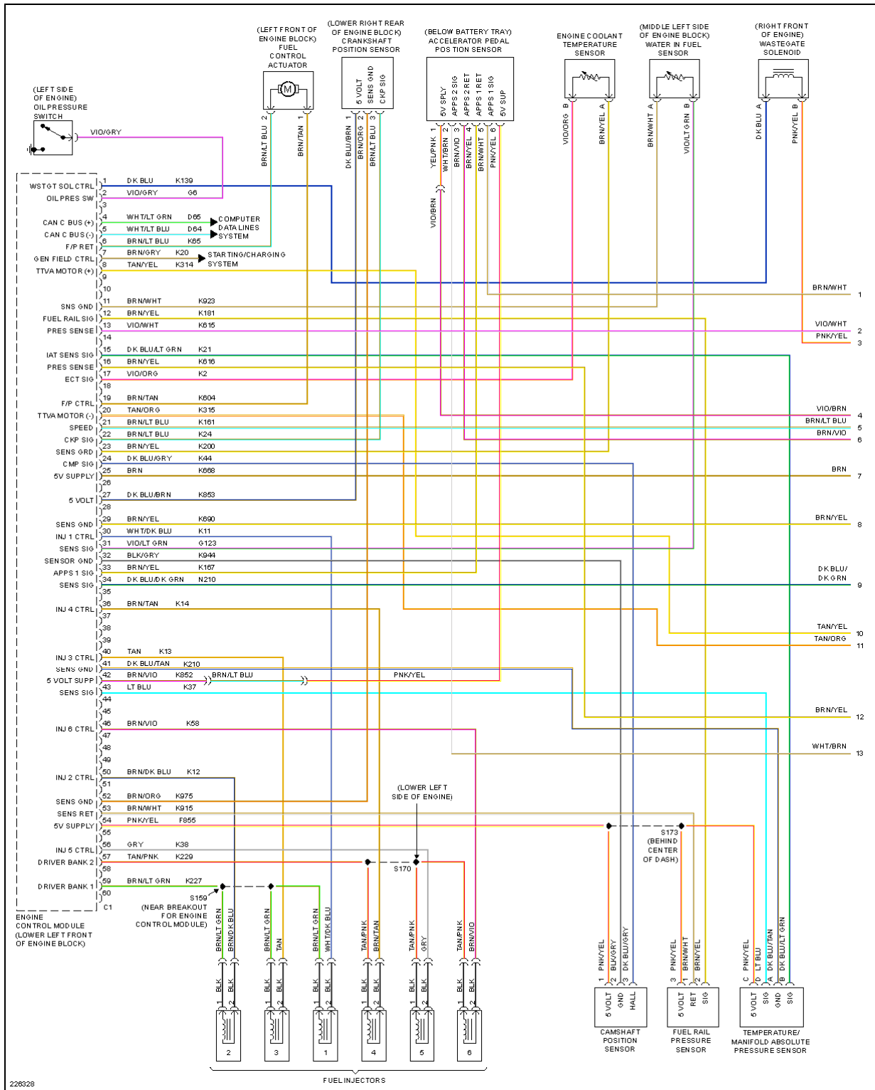
Fig. 17: 5.9L Diesel, Engine Performance Circuit (1 of 4)
